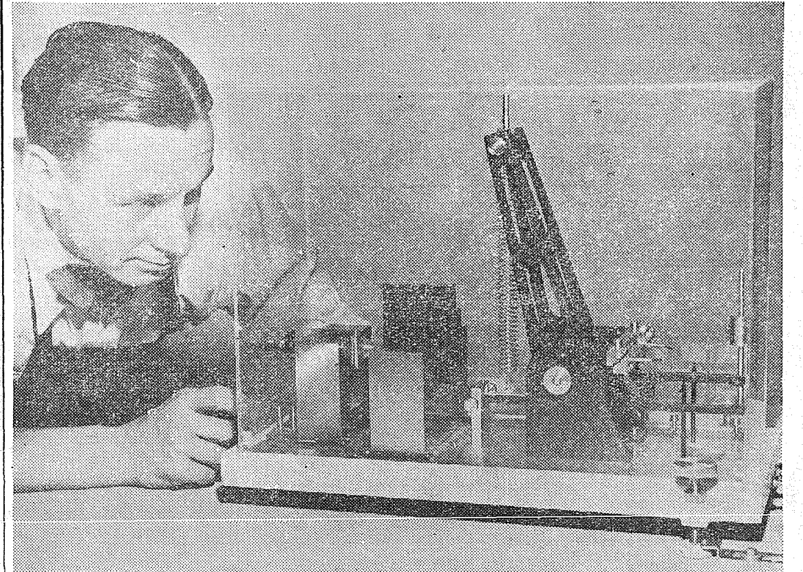
Dr. Eijo Vesanen, University of Washington seismologist, examines a seismometer, part of a new seismograph installation at the University that will make the station one of the best equipped in the nation. The apparatus is several hundred times more efficient than the 1905 model it replaces on the campus.
