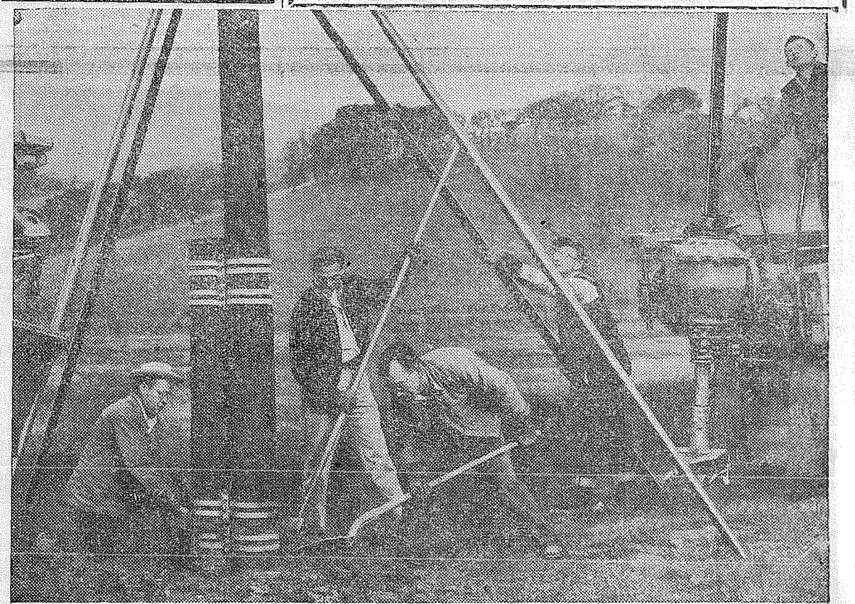
"Pole stubbers" at work: Inspection has revealed a pole which shows damage at the ground line. Now, reinforced with a short length, it will be strong as new, and we'll have saved much of the cost of a new pole.
