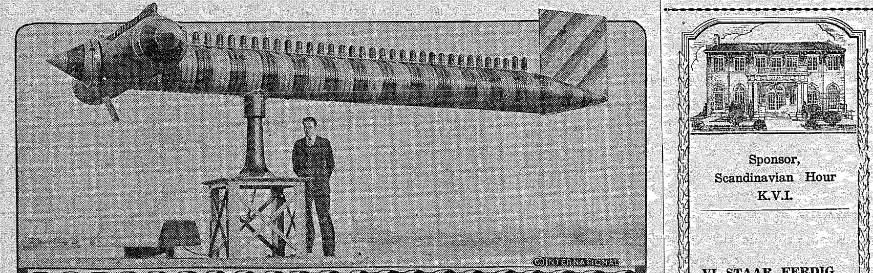
This is the newly installed wind tee atop a hangar at the central airport in Camden, N. J., replacing the outmoded wind sock. Rows of lights operated by pressure denote the force of the wind and are visible at a distance of three miles.
