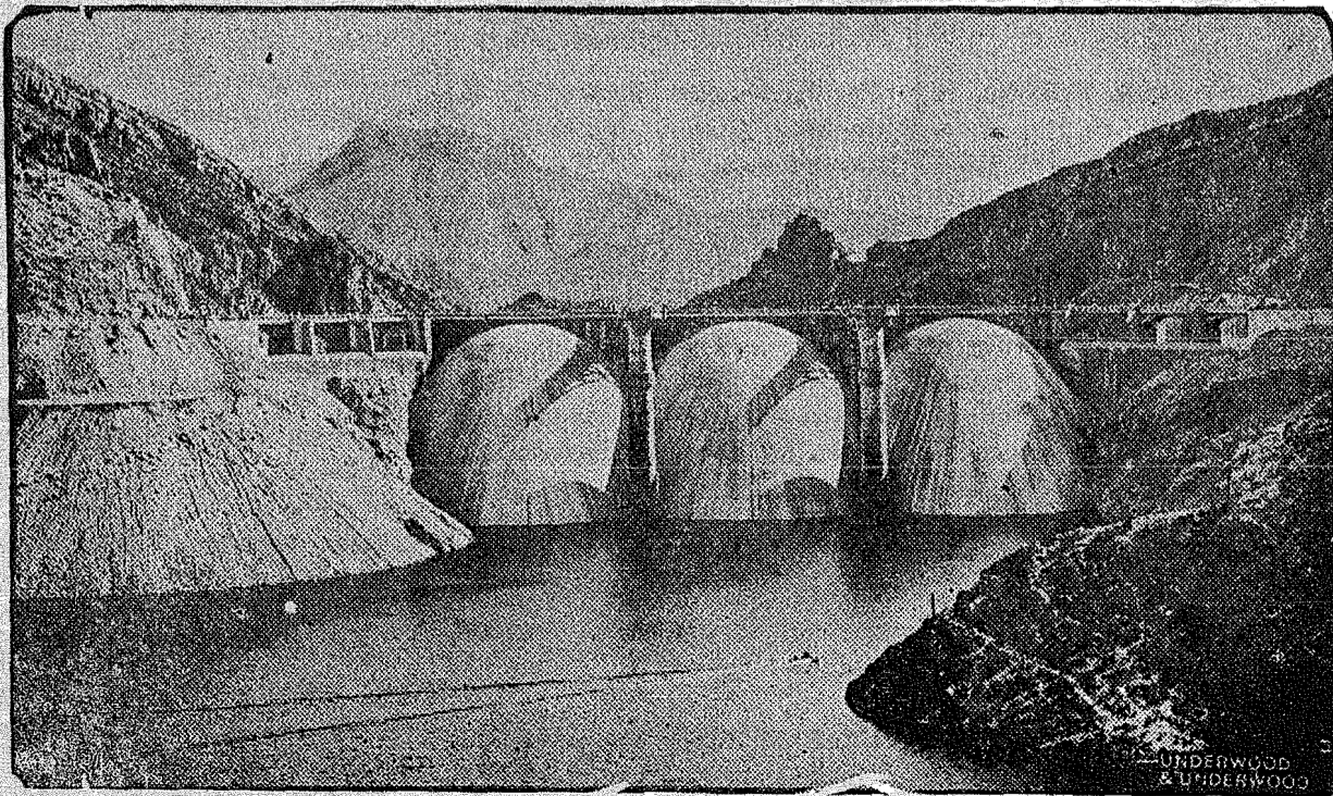
A new picture of the Coolidge dam in Arizona which reveals the impressiveness of the only multiple-dome dam in the world. It is situated about 135 miles southeast of Phoenix, and will serve to irrigate 100,000 acres of land along the Gila river.
