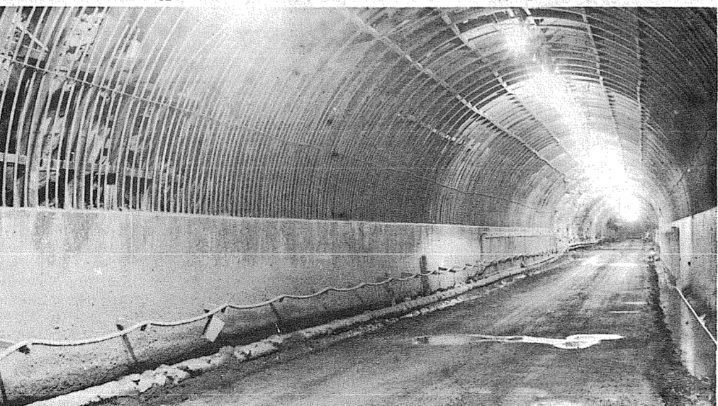
THIS CAVERNOUS TUNNEL leads into the heart of Cheyenne Mountain where NORAD's underground Combat Operations Center is under construction. A three-story building inside the mountain will house electronic equipment needed to maintain the constant surveillance on North America's aerospace boundaries and provide data the NORAD staff would use to conduct the aerospace defense of this continent should the need arise.
