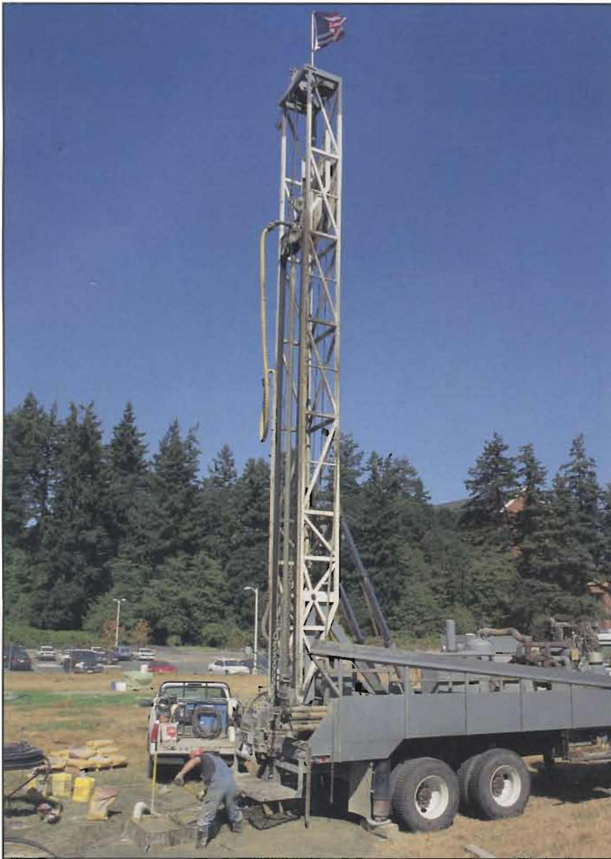
Drilling for a geothermal heating and cooling system is part of the first phase in the construction of the Morken Center for Learning and Technology.
